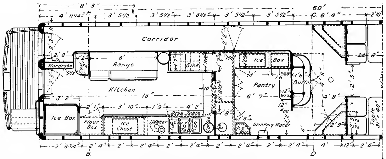
Fig. 475. Plan of Kitchen, Pantry and Buffet.
